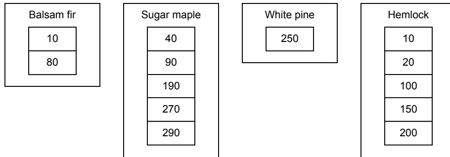
Figure 0 – Example of a set of cohorts for a set (based on Table 1 in He1999).
