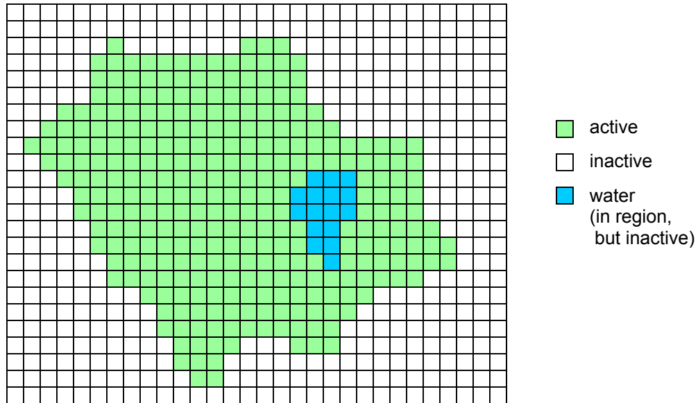
Figure 0 – Region of interest on a landscape.
