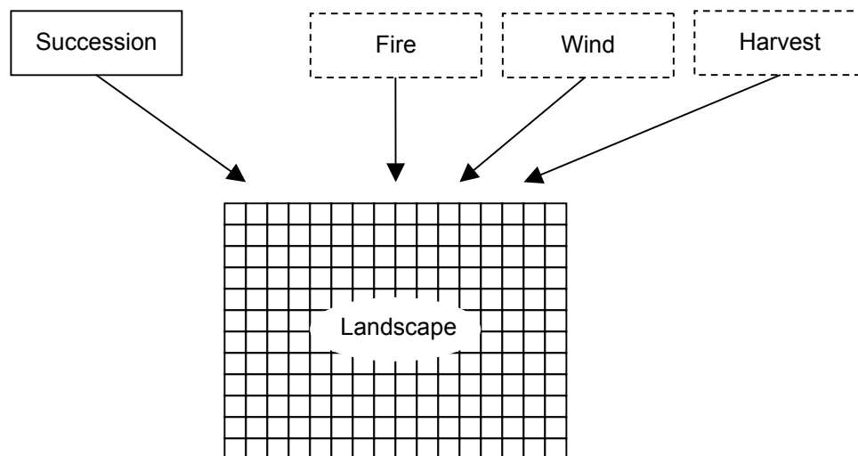
Figure 0 – Ecological processes modify landscape.
