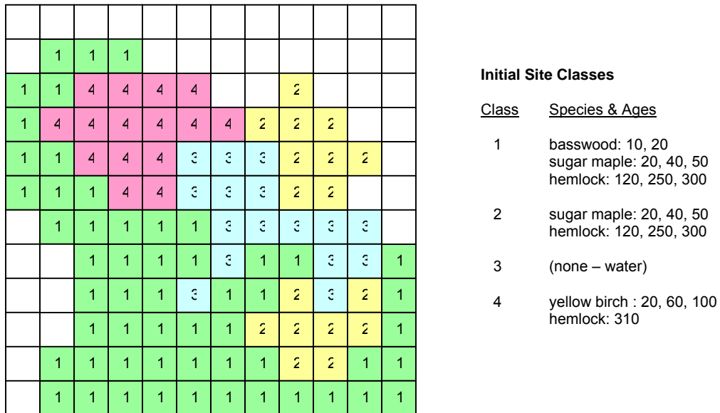
Figure 0 – Example of a site initialization map.
